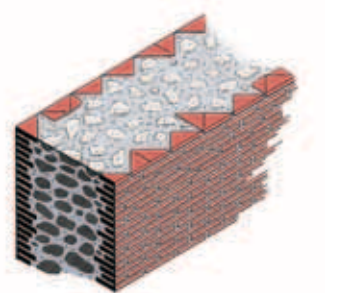
V. Opus testaceum
